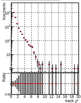
N of reco track vs. \chi^2 — Global_mkFit1000o_RECO — Global_mkFit1000o_RECO
