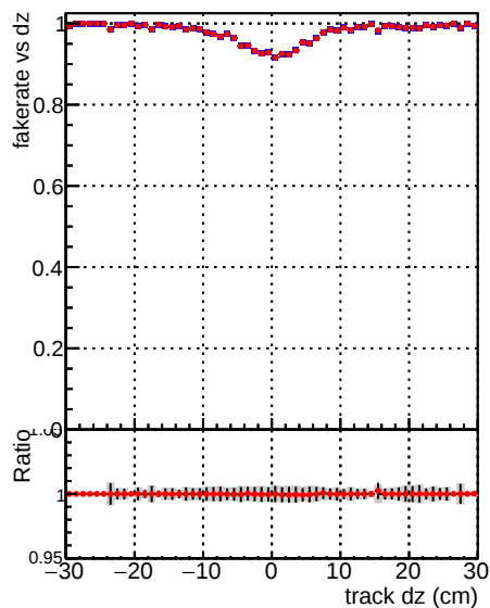
—•— DQM_V0001_R0000000001_Global_mkFit1000o_RECO —•— DQM_V0001_R0000000001_Global_mkFit1000o_RECO
