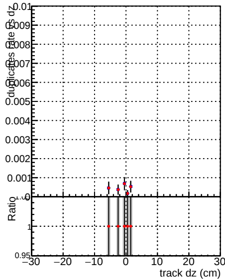
DQM_V0001_R0000000001 Global mkFit1000o RECO Fake rate vs dz Duplicates Rate vs dz Pileup rate vs dz
