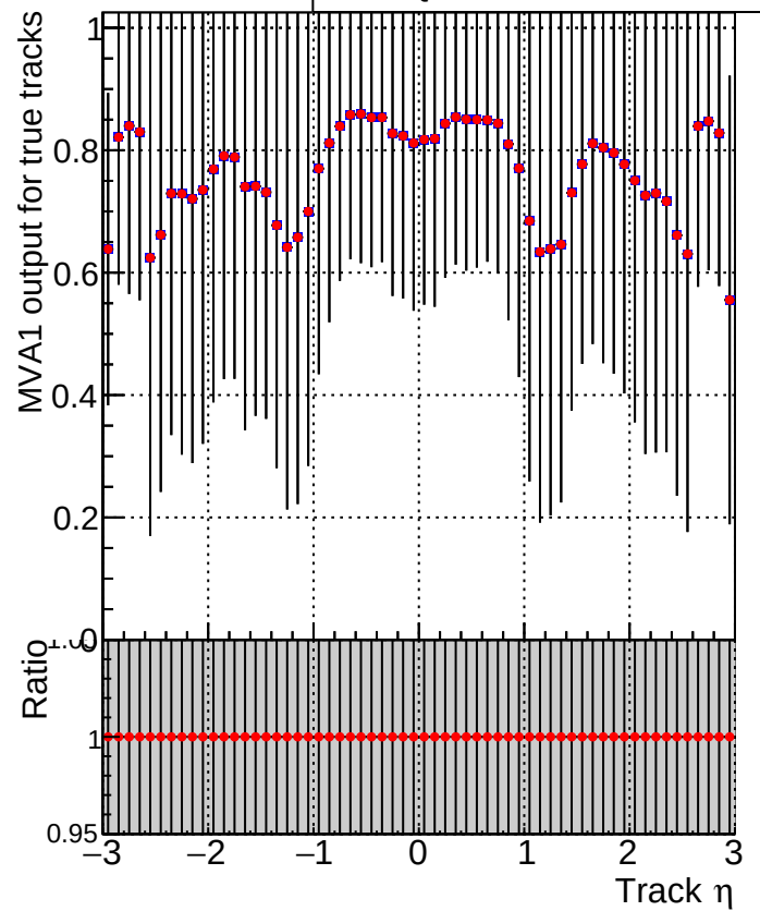
MVA1 of associated tracks (recoToSim) vs. track \eta Legend: Grey histogram: DQM_V0001_R000000001_Global_mkFit1000o_RECO Red stars: DQM_V0001_R000000001_Global_mkFit1000_RECO
