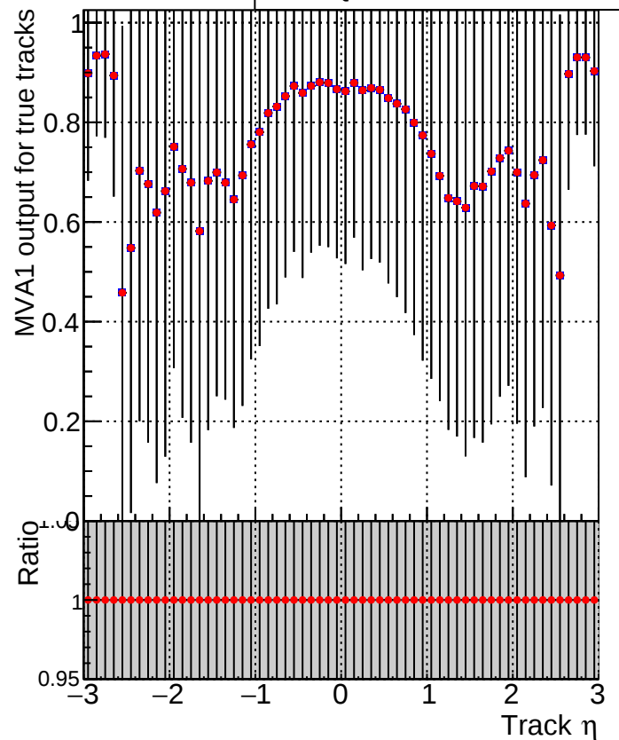
MVA1 of associated tracks (recoToSim) vs. track \eta Legend: █ DQM_V0001_R000000001_Global_mkFit1000o_RECO ● DQM_V0001_R000000001_Global_mkFit1000_RECO
