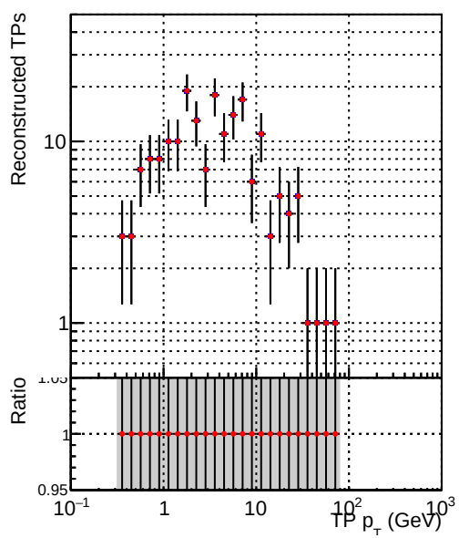
Legend: DQM_V0001_R000000001_Global_mkFit1000o_RECO
