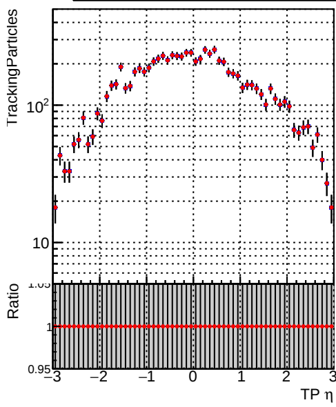
Legend: DQM_V0001_R000000001_Global_mkFit1000o_RECO
