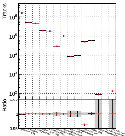
DQM_V0001_R000000001_Global_mkFit1000o_RECO
