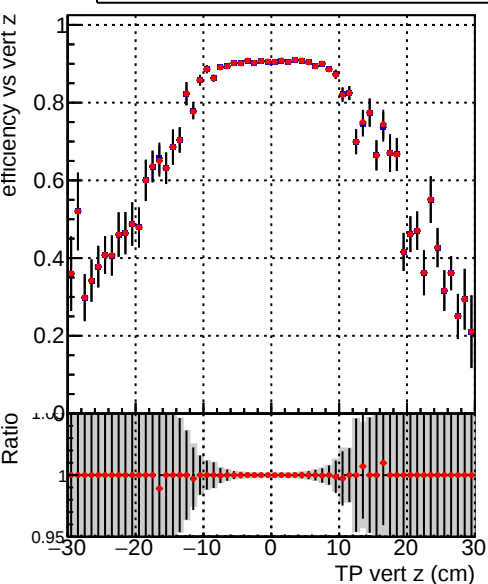
Efficiency
