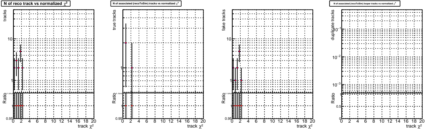
N of reco track vs. \chi^2 DQM_V0001_R0000000001_Global_mkFit1000o_RECO DQM_V0001_R0000000001_Global_mkFit1000o_RECO
