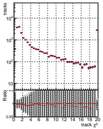
N of reco track vs. - blue line: DQM_V0001_R000000001_Global_mkFit1000o_RECO - red line: DQM_V0001_R000000001_Global_mkFit1000_RECO
