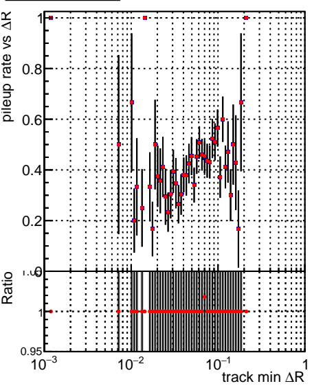
█ ● DQM_V0001_R000000001_Global_mkFit1000o_RECO █ ● DQM_V0001_R000000001_Global_mkFit1000_RECO
