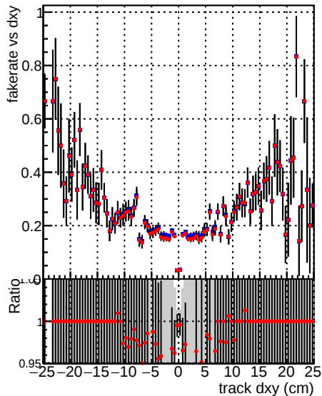
—●— DQM_V0001_R0000000001_Global_mkFit1000o_RECO —●— DQM_V0001_R0000000001_Global_mkFit1000_RECO
