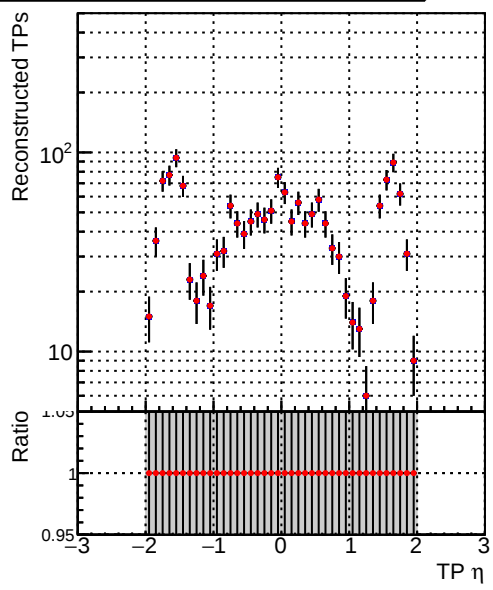
Legend: DQM_V0001_R0000000001_Global_mkFit1000o_RECO
