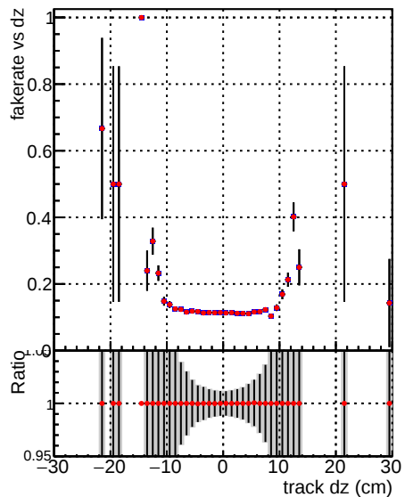
Fake rate vs d DQM_V0001_R0000000001 Global mkFit1000o RECO DQM_V0001_R0000000001 Global mkFit1000 RECO
