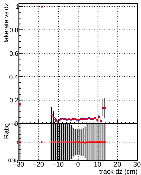
Fake rate vs dz Global mkFit1000o RECO DQM_V0001_R0000000001 Global mkFit1000 RECO DQM_V0001_R0000000001
