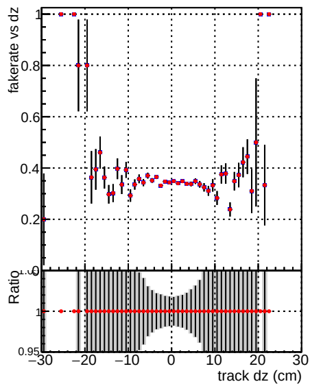
Fake rate vs dz Global mkFit1000o RECO Global mkFit1000 RECO
