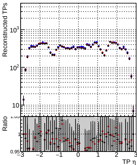
● DQM_original_step2_ttbbar-phase1-newgeom ● DQM_pixelCPETemplate_step2_ttbbar-phase1-newgeom ● DQM_pixelCPETemplateCutChiSquareNew_step2_ttbbar-phase1-newgeom
