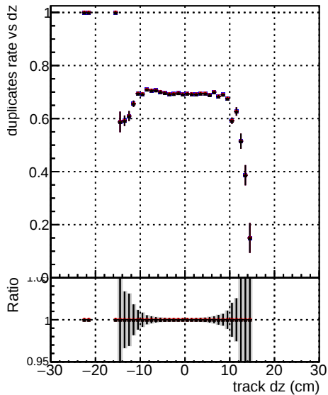
DOM original_step2_tbar-phase1-newgeom DOM pixelCPEtemplate_step2_tbar-phase1-newgeom DOM pixelCPEtemplatecurchisquareNew_step2_tbar-phase1-newgeom
