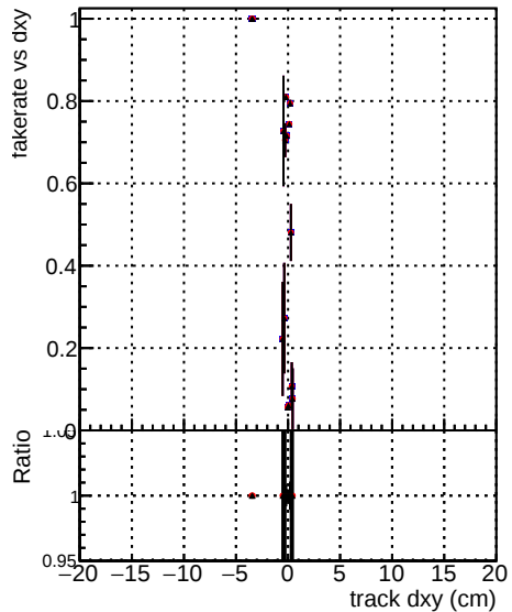
DOM original_step2_tbar-phase1-newgeom DOM pixelCPEtemplate_step2_tbar-phase1-newgeom DOM pixelCPEtemplatecurchisquareNew_step2_tbar-phase1-newgeom
