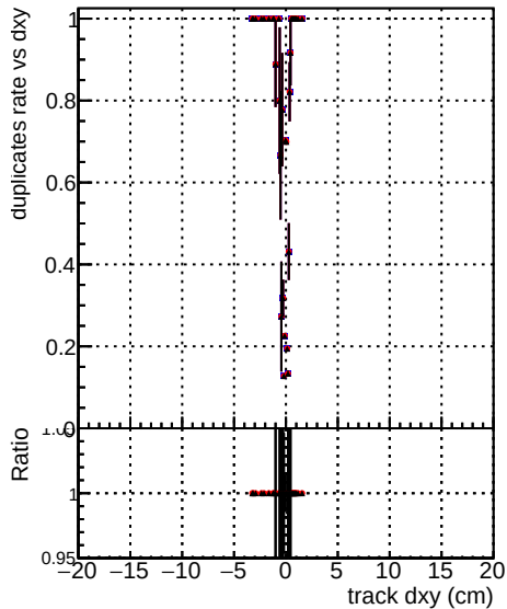
DOM original_step2_tbar-phase1-newgeom DOM pixelCPE_template_step2_tbar-phase1-newgeom DOM pixelCPE_template_cut_chiSquareNew_step2_tbar-phase1-newgeom
