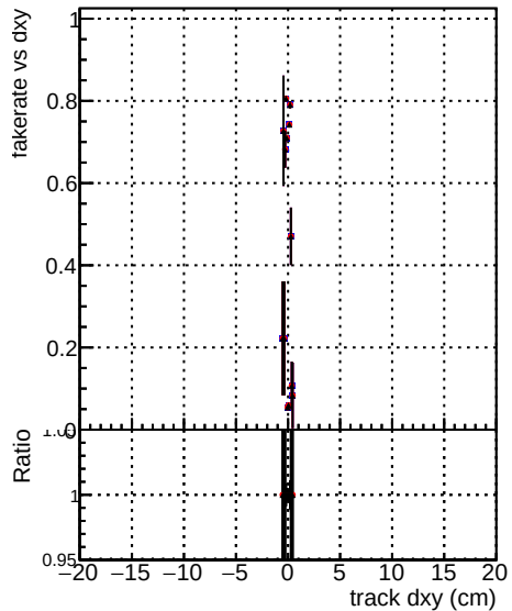
DOM original_step2_tbar-phase1-newgeom DOM pixelCPE_template_step2_tbar-phase1-newgeom DOM pixelCPE_template_cut_chiSquareNew_step2_tbar-phase1-newgeom
