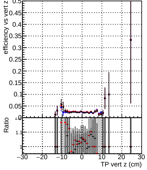
Efficiency vs vert z —●— DQM_original_step2_ttbarm-phase1-newgeom —●— DQM_pixelCPETemplate_step2_ttbarm-phase1-newgeom —●— DQM_pixelCPETemplateCutChiSquareNew_step2_ttbarm-phase1-newgeom
