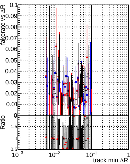
—•— DQM_original_step2_ttbar-phase1-newgeom —•— DQM_pixelCPETemplate_step2_ttbar-phase1-newgeom —•— DQM_pixelCPETemplateCutChiSquareNew_step2_ttbar-phase1-newgeom
