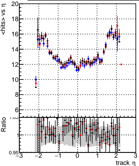
mean hits vs \eta — DQM_original_step2_ttbar-phase1-newgeom — DQM_pixelCPETemplate_step2_ttbar-phase1-newgeom — DQM_pixelCPETemplateCutChiSquareNew_step2_ttbar-phase1-newgeom
