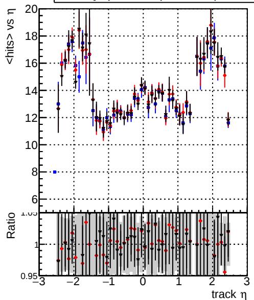
DQM_original_step2_ttbar-phase1-newgeom DQM_pixelCPETemplate_step2_ttbar-phase1-newgeom DQM_pixelCPETemplateCutChiSquareNew_step2_ttbar-phase1-newgeom mean hits
