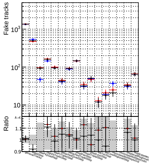
Number of tracks vs collection DQM_original_step2_ttbar-phase1-newgeom DQM_pixelCPETemplate_step2_ttbar-phase1-newgeom DQM_pixelCPETemplateCutChiSquareNew_step2_ttbar-phase1-newgeom
