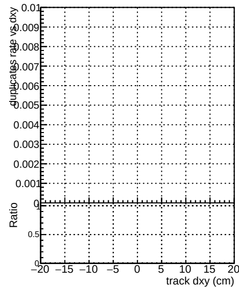
ttbar-phase1-newgeom SquareNew_step2_ttbar-phase1-newgeom
