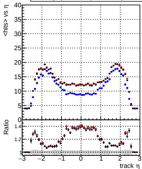
mean hits vs \eta Legend: — DQM_original_step2_ttbar-phase1-newgeom — DQM_pixelCPETemplate_step2_ttbar-phase1-newgeom — DQM_pixelCPETemplateCutChiSquareNew_step2_ttbar-phase1-newgeom
