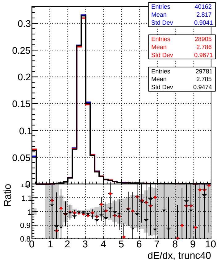
— DQM_original_step2_ttbar-phase1-newgeom — DQM_pixelCPETemplate_step2_ttbar-phase1-newgeom — DQM_pixelCPETemplateCutChiSquareNew_step2_ttbar-phase1-newgeom
