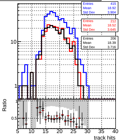
mean hit — DQM_original_step2_ttbbar-phase1-newgeom — DQM_pixelCPETemplate_step2_ttbbar-phase1-newgeom — DQM_pixelCPETemplateCutChiSquareNew_step2_ttbbar-phase1-newgeom
