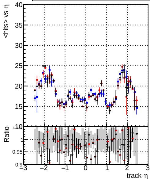
mean hit — DQM_original_step2_ttbbar-phase1-newgeom — DQM_pixelCPETemplate_step2_ttbbar-phase1-newgeom — DQM_pixelCPETemplateCutChiSquareNew_step2_ttbbar-phase1-newgeom
