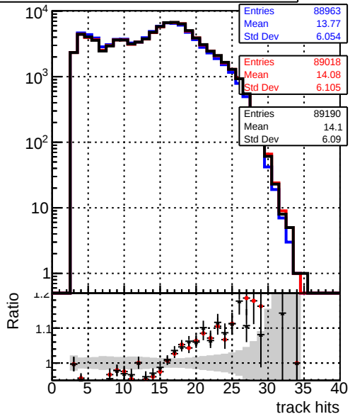
mean hit — DQM_original_step2_ttbar-phase1-newgeom — DQM_pixelCPETemplate_step2_ttbar-phase1-newgeom — DQM_pixelCPETemplateCutChiSquareNew_step2_ttbar-phase1-newgeom
