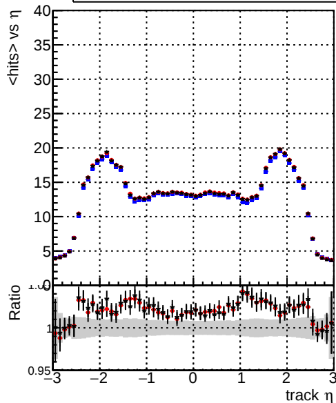
mean hit — DQM_original_step2_ttbar-phase1-newgeom — DQM_pixelCPETemplate_step2_ttbar-phase1-newgeom — DQM_pixelCPETemplateCutChiSquareNew_step2_ttbar-phase1-newgeom
