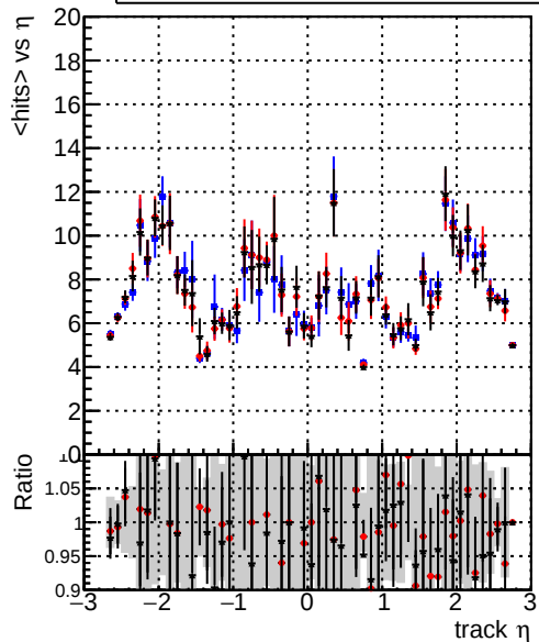
mean hit — DQM_original_step2_ttbar-phase1-newgeom — DQM_pixelCPETemplate_step2_ttbar-phase1-newgeom — DQM_pixelCPETemplateCutChiSquareNew_step2_ttbar-phase1-newgeom
