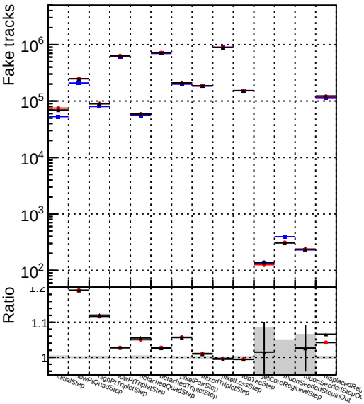
Number Model 1 DQM_pixelCPETemplate_step2_ttbar-phase1-newgeom 2 DQM_pixelCPETemplateCutChiSquareNew_step2_ttbar-phase1-newgeom
