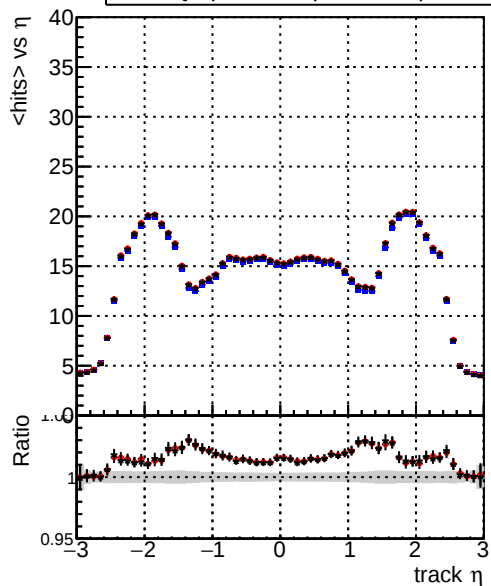
DQM_original_step2_ttbar-phase1-newgeom DQM_pixelCPETemplate_step2_ttbar-phase1-newgeom DQM_pixelCPETemplateCutChiSquareNew_step2_ttbar-phase1-newgeom mean hits
