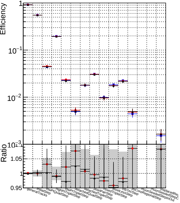
DQM_original_step2_ttbar-phase1-newgeom DQM_pixelICPETemplate_step2_ttbar-phase1-newgeom DQM_pixelICPETemplateCutChiSquareNew_step2_ttbar-phase1-newgeom
