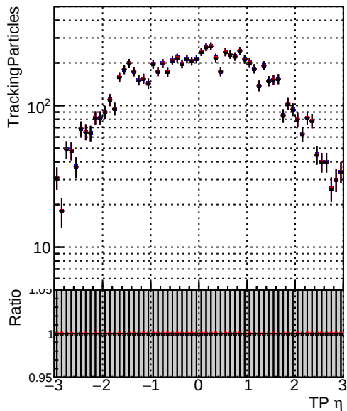
— DQM_original_step2_ttbbar-phase1-newgeom — DQM_pixelCPETemplate_step2_ttbbar-phase1-newgeom — DQM_pixelCPETemplateCutChiSquareNew_step2_ttbbar-phase1-newgeom
