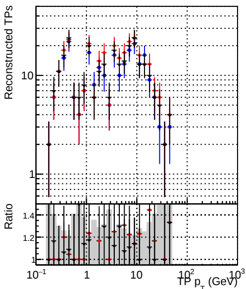
— DQM_original_step2_ttbbar-phase1-newgeom — DQM_pixelCPETemplate_step2_ttbbar-phase1-newgeom — DQM_pixelCPETemplateCutChiSquareNew_step2_ttbbar-phase1-newgeom
