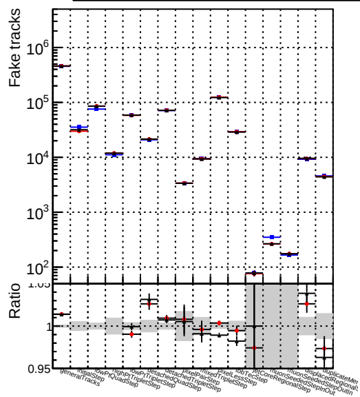
Number Legend 1 DQM_pixelCPETemplate_step2_ttbar-phase1-newgeom 2 DQM_pixelCPETemplateCutChiSquareNew_step2_ttbar-phase1-newgeom
