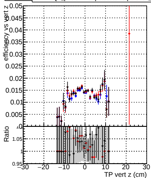
Efficiency vs. TP vert z —●— DQM_original_step2_ttbbar-phase1-newgeom —●— DQM_pixelCPETemplate_step2_ttbbar-phase1-newgeom —●— DQM_pixelCPETemplateCutChiSquareNew_step2_ttbbar-phase1-newgeom
