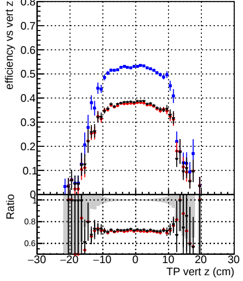
Efficiency vs vert z — DQM_original_step2_ttbare-phase1-newgeom — DQM_pixelCPETemplate_step2_ttbare-phase1-newgeom — DQM_pixelCPETemplateCutChiSquareNew_step2_ttbare-phase1-newgeom
