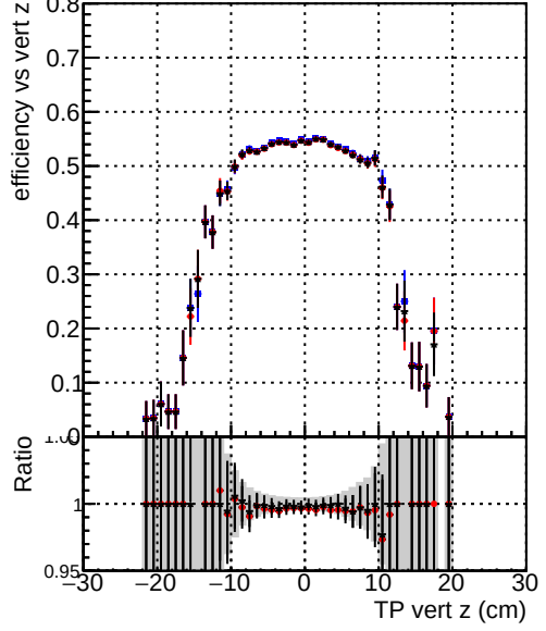
Efficiency vs. TP vert z (cm) —●— DQM_original_step2_ttbare-phase1-newgeom —+— DQM_pixelCPETemplate_step2_ttbare-phase1-newgeom —x— DQM_pixelCPETemplateCutChiSquareNew_step2_ttbare-phase1-newgeom
