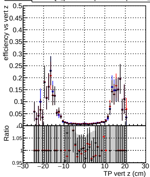
Efficiency vs vert z —●— DQM_original_step2_ttbar-phase1-newgeom —●— DQM_pixelCPETemplate_step2_ttbar-phase1-newgeom —●— DQM_pixelCPETemplateCutChiSquareNew_step2_ttbar-phase1-newgeom
