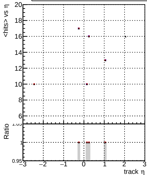
mean hits vs \eta DQM_original_step2_ttbar-phase1-newgeom DQM_pixelCPETemplate_step2_ttbar-phase1-newgeom DQM_pixelCPETemplateCutChiSquareNew_step2_ttbar-phase1-newgeom
