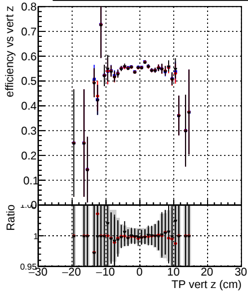
Efficiency vs. TP vert z (cm) — DQM_original_step2_ttbbar-phase1-newgeom — DQM_pixelCPETemplate_step2_ttbbar-phase1-newgeom — DQM_pixelCPETemplateCutChiSquareNew_step2_ttbbar-phase1-newgeom
