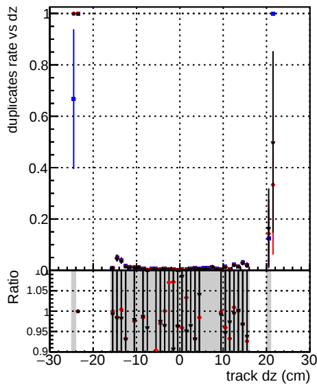
DOM original step2 ttbar-phase1-newgeom DOM pixelCPEtemplate step2 ttbar-phase1-newgeom DOM pixelCPEtemplateCutChiSquareNew step2 ttbar-phase1-newgeom
