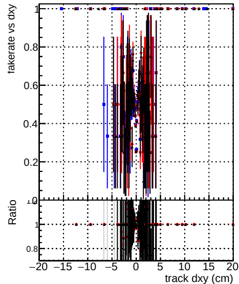
DOM original step2 ttbar-phase1-newgeom DOM pixelCPETemplate step2 ttbar-phase1-newgeom DOM pixelCPETemplateCutChiSquareNew step2 ttbar-
