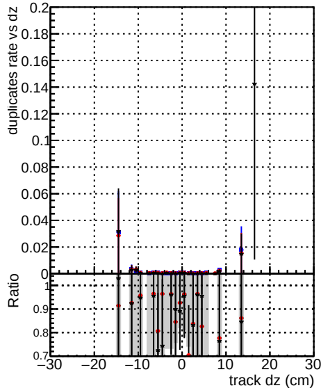
ttbar-phase1-newgeom SquareNew_step2_ttbar-phase1-newgeom
