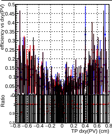
Efficiency vs Dxy(PV) Legend: DQM_original_step2_ttbar-phase1-newgeom DQM_pixelCPETemplate_step2_ttbar-phase1-newgeom DQM_pixelCPETemplateCutChiSquareNew7_step2_ttbar-phase1-newgeom
