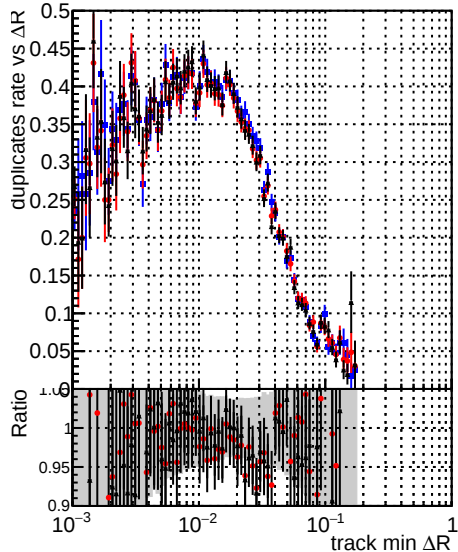
—■— DQM_original_step2_ttbar-phase1-newgeom —●— DQM_pixelCPETemplate_step2_ttbar-phase1-newgeom —▲— DQM_pixelCPETemplateCutChiSquareNew7_step2_ttbar-phase1-newgeom
