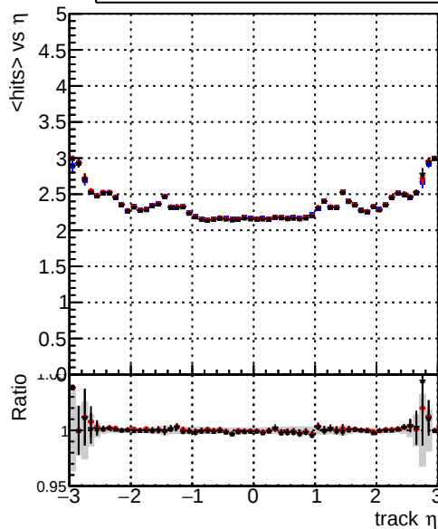
mean hits vs \eta DQM_original_step2_ttbar-phase1-newgeom DQM_pixelCPETemplate_step2_ttbar-phase1-newgeom DQM_pixelCPETemplateCutChiSquareNew7_step2_ttbar-phase1-newgeom
