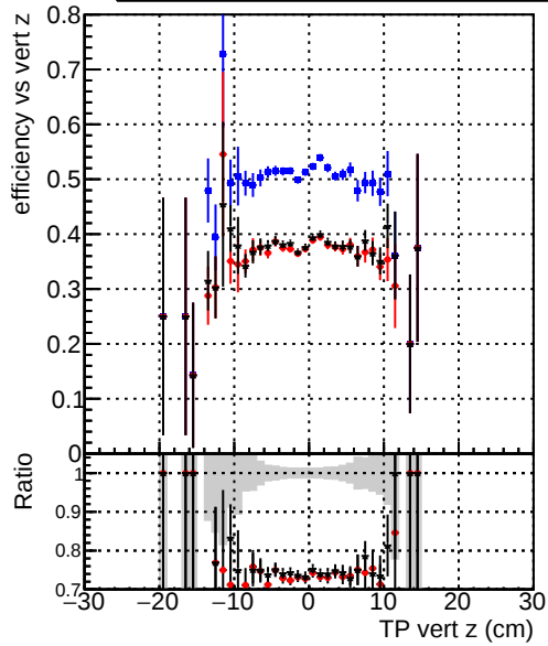
Efficiency vs. TP vert z (cm) — DQM_original_step2_ttbar-phase1-newgeom — DQM_pixelCPETemplate_step2_ttbar-phase1-newgeom — DQM_pixelCPETemplateCutChiSquareNew7_step2_ttbar-phase1-newgeom
