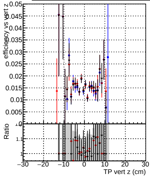
Efficiency vs. TP vert z —●— DQM_original_step2_ttbar-phase1-newgeom —●— DQM_pixelCPETemplate_step2_ttbar-phase1-newgeom —●— DQM_pixelCPETemplateCutChiSquareNew7_step2_ttbar-phase1-newgeom
