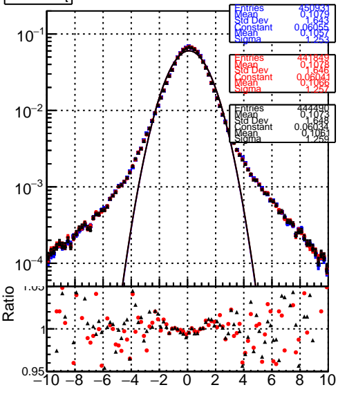
■ BDM original_step2_tbar-phase1-newgeom ■ BDM pixelCPE_TemplateCutsNew_step2_tbar-phase1-newgeom ■ BDM TemplateCutsNew_step2_tbar-phase1-newgeom
